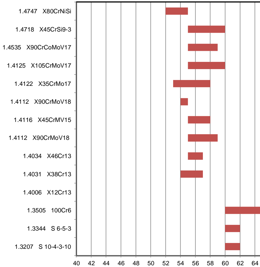
erreichbare Härte SH in HRC achievable hardness SH in HRC
