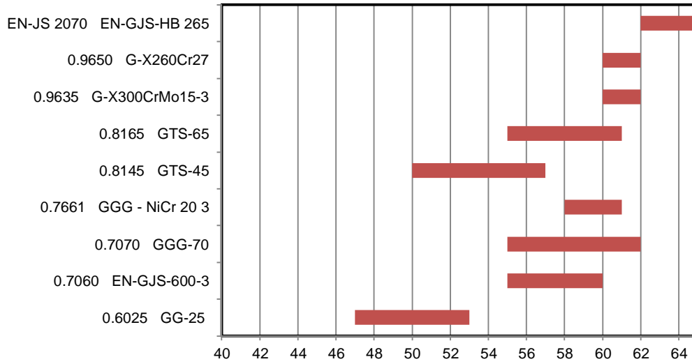
erreichbare Härte SH in HRC achievable hardness SH in HRC
